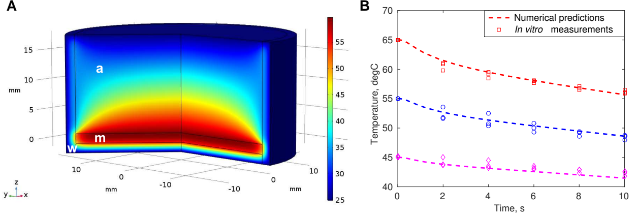
Figure S3: Comparison of in silico and in vitro models of heat transfer in a 6-well plate. (A) Temperature distribution in the medium (m), plate wall (w) and air (a) at 5 seconds after the initial medium temperature of 65°C. (B) Associated cooling curves predicted by the mathematical model (at mid-depth z = \delta/2 , r = 0 ; dashed lines) and measured at varying positions in vitro (symbols).
